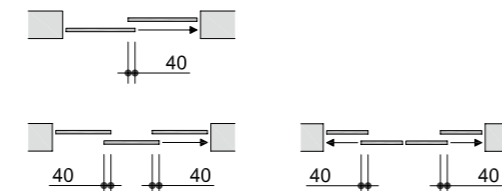
Piastre copri-carrello Trolley-cover plates
